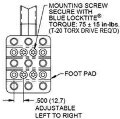
FOOT PAD DETAIL
